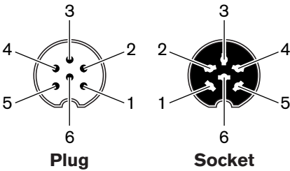
Figure 4.2: Plug and socket pin numbers
