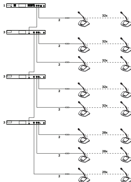
Figure 4.6: Example setup for a large system with 35 m of extension cable connected to the trunk and each tap-off
