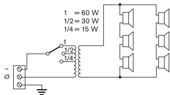
Fig. 5: Circuit diagram
